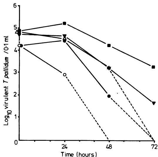
FIG 1 The fall in concentration of virulent T pallidum (per 0.1 ml) in media with different redox potentials: ■ anaerobic tubes: average redox potential, -387 mV (E cal ); Δ 20-ml tubes: average redox potential, -325 mV (E cal ); ▼ 10-ml tubes: average redox potential, -268 mV (E cal ); ● 5-ml tubes: average redox potential, -166 mV (E cal ); and ○ 3-ml tubes: average redox potential, -94 mV (E cal ).
